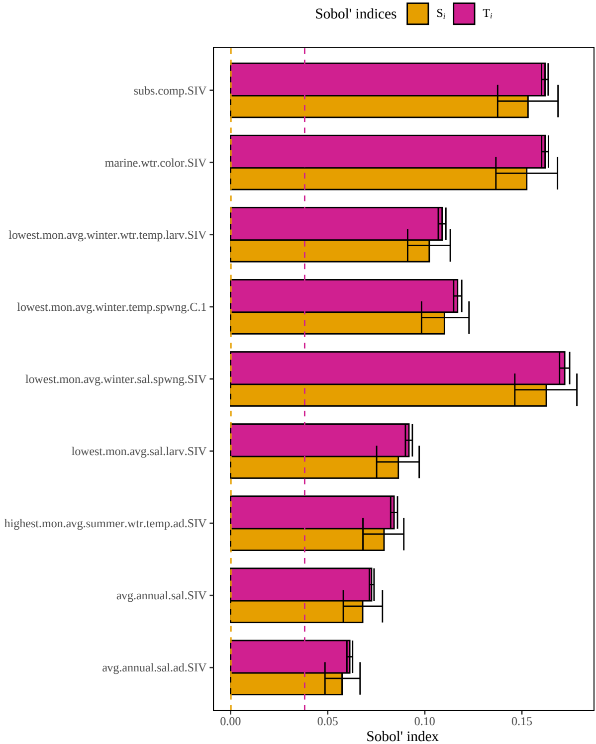
Figure 5. Results of a sensitivity analysis for the gulfmenhadenMarine model based on a geometric mean structure. Dashed lines represent baseline numerical approximation error for S_i and T_i ( i.e. , dummy variables).
