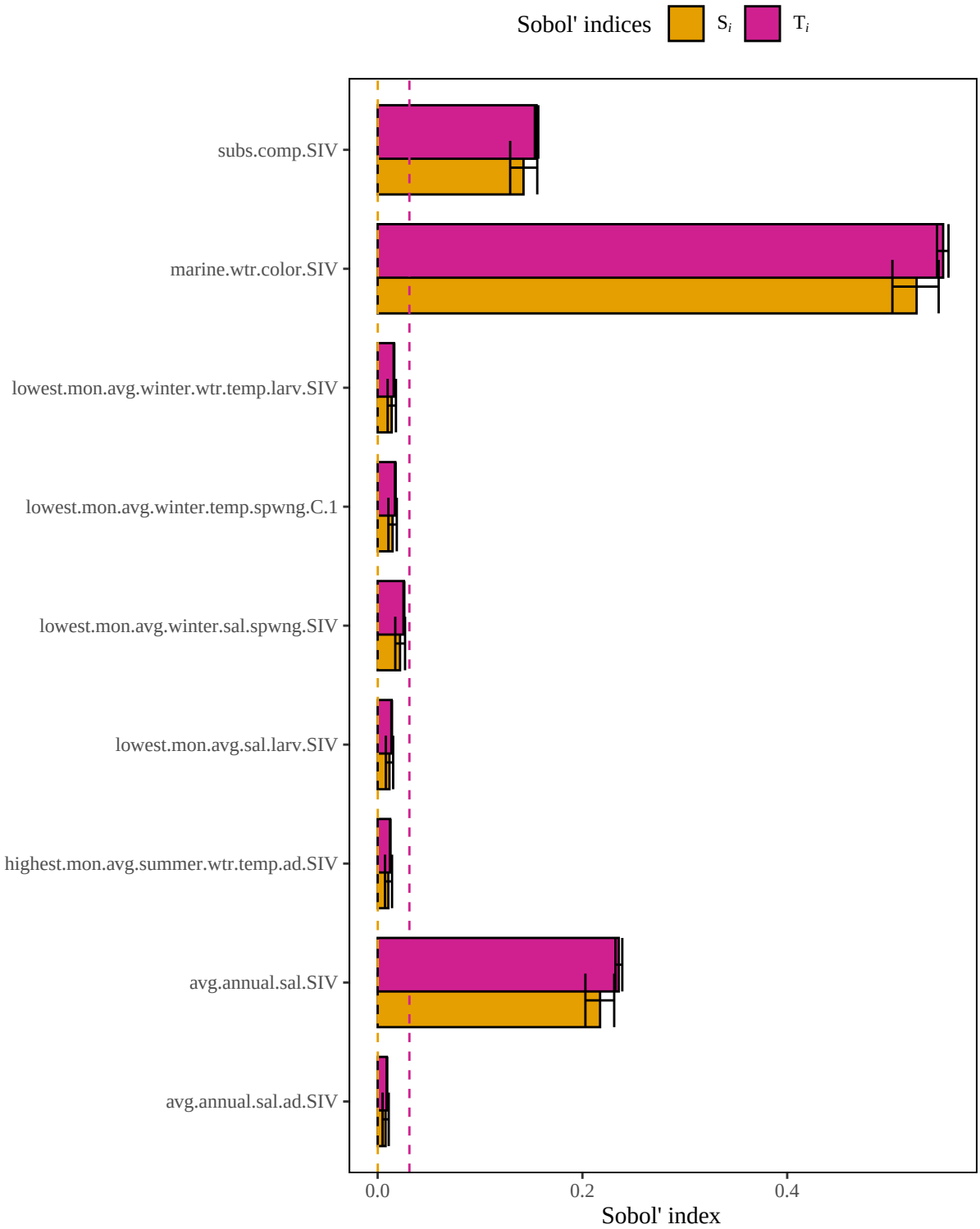
Figure 3. Results of a sensitivity analysis for the gulfmenhadenMarine model based on the original author-specified model outlined in Christmas et al. (1982). Dashed lines represent baseline numerical approximation error for S_i and T_i ( i.e. , dummy variables).
