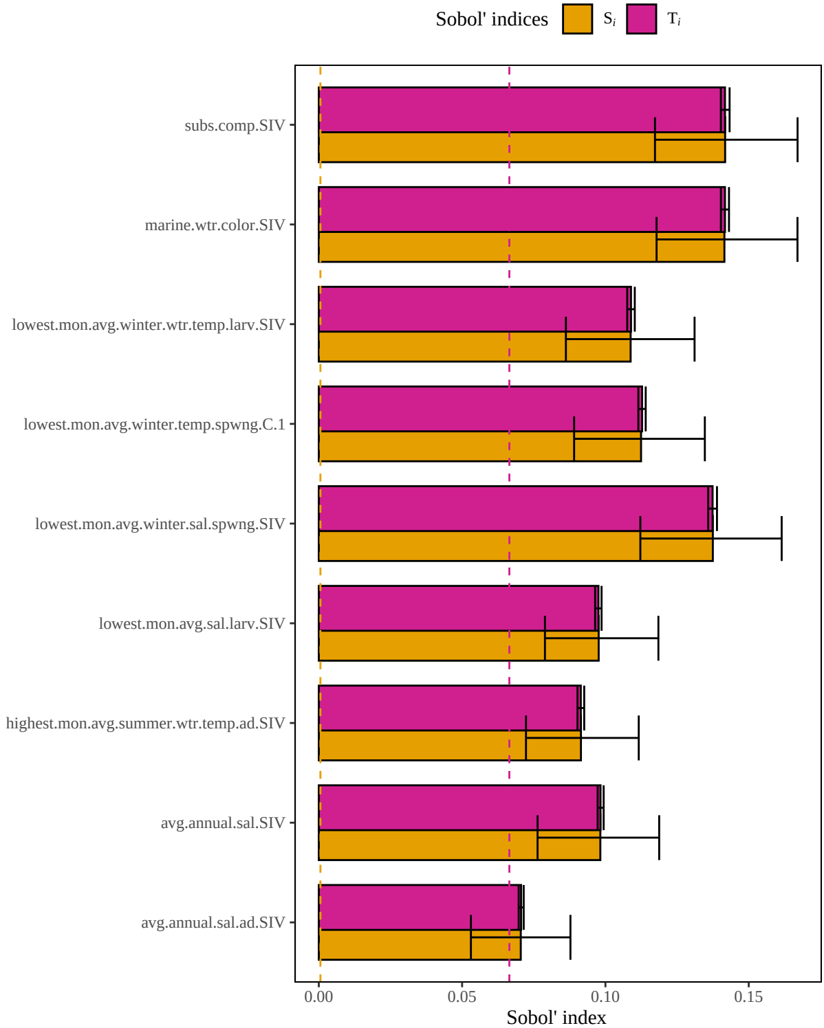
Figure 4. Results of a sensitivity analysis for the gulfmenhadenMarine model based on an arithmetic mean structure. Dashed lines represent baseline numerical approximation error for S_i and T_i ( i.e. , dummy variables).
