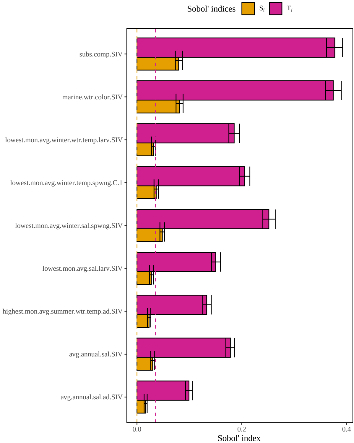
Figure 7. Results of a sensitivity analysis for the gulfmenhadenMarine model based on a multiplicative mean structure. Dashed lines represent baseline numerical approximation error for S_i and T_i ( i.e. , dummy variables).
